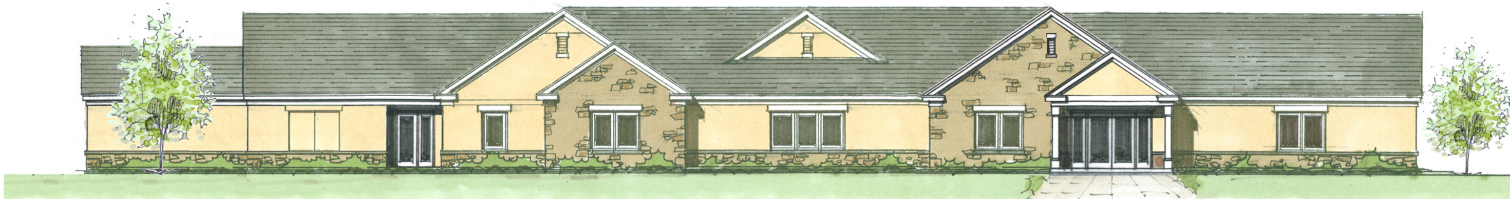
FRONT ELEVATION 1/8" = 1'-0"
